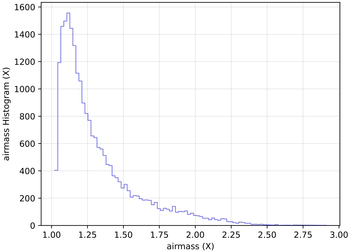
ddf_loaded_fl2_v3.4_10yrs Yr 1 g band: airmass Histogram
