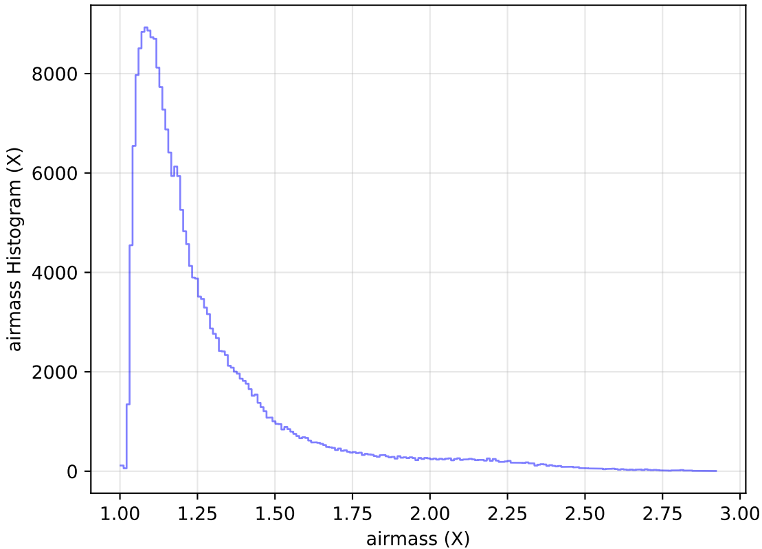
ddf_loaded_fl2_v3.4_10yrs Yr 1 all bands: airmass Histogram
