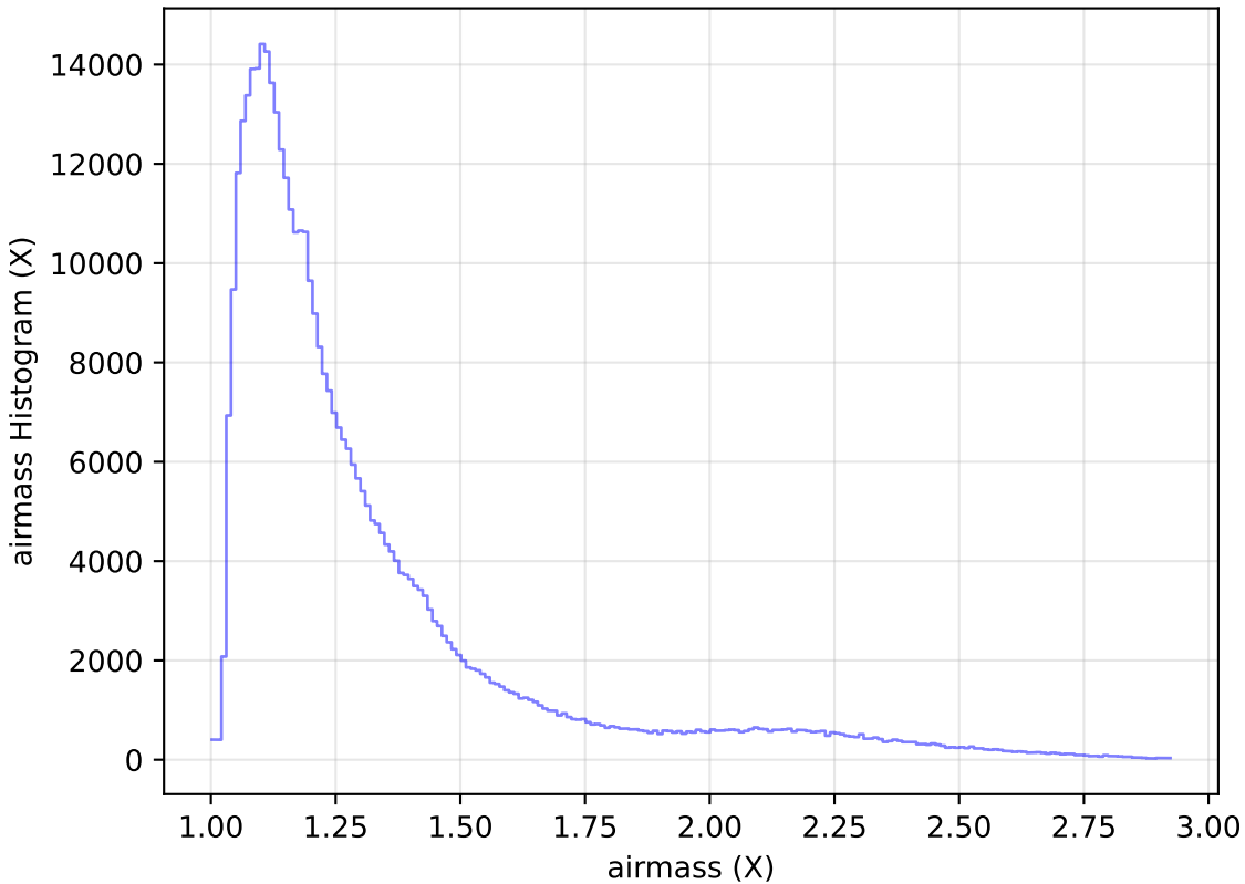
ddf_loaded_fl2_v3.4_10yrs WFD z band: airmass Histogram
