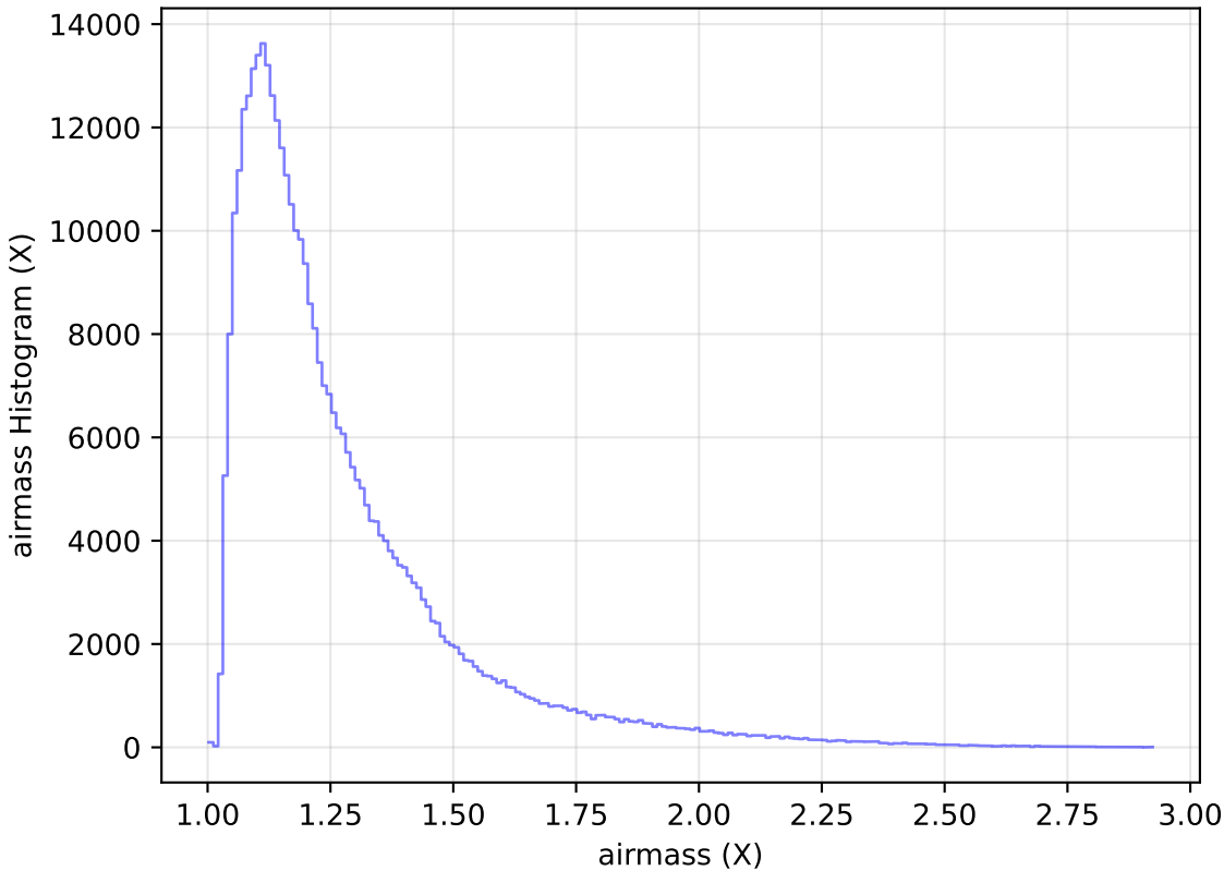
ddf_loaded_fl2_v3.4_10yrs WFD y band: airmass Histogram
