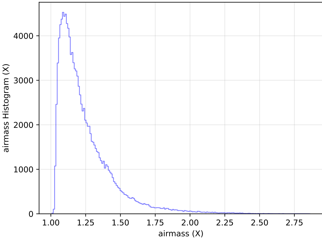
ddf_loaded_fl2_v3.4_10yrs WFD u band: airmass Histogram
