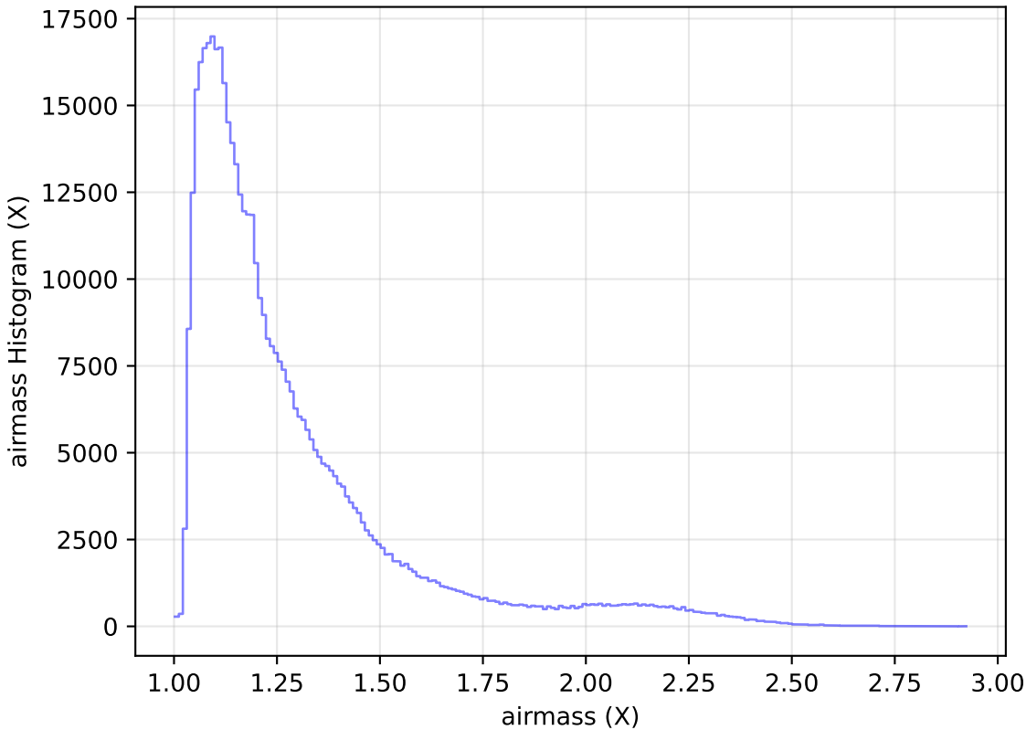
ddf_loaded_fl2_v3.4_10yrs WFD r band: airmass Histogram
