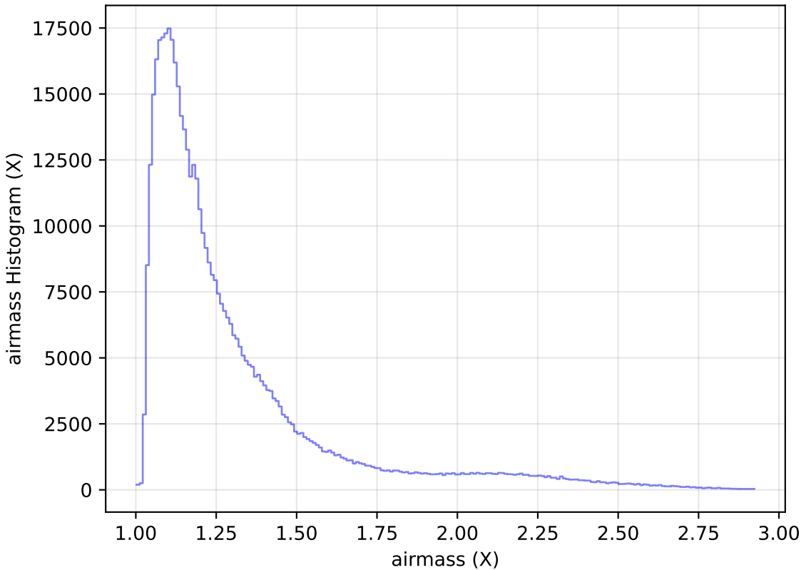
ddf_loaded_fl2_v3.4_10yrs WFD i band: airmass Histogram
