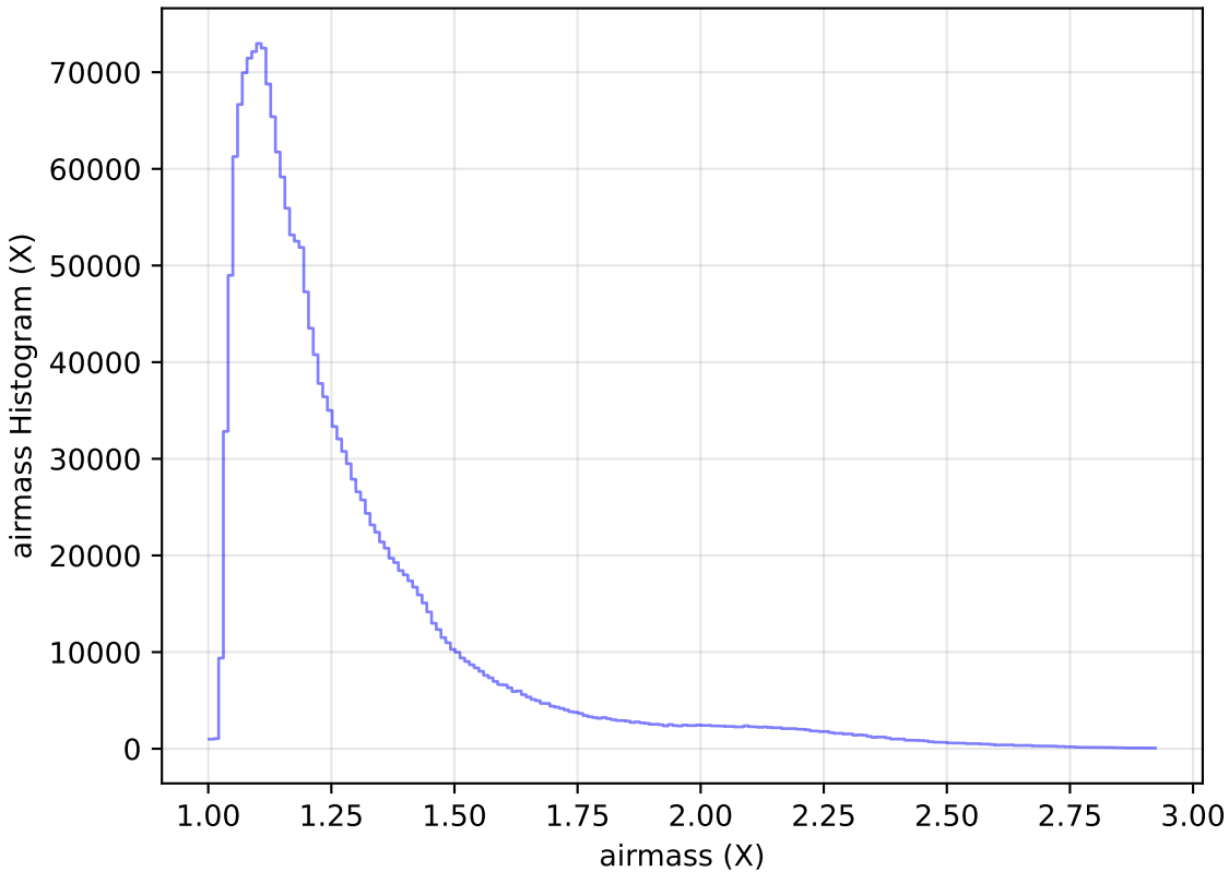
ddf_loaded_fl2_v3.4_10yrs WFD all bands: airmass Histogram
