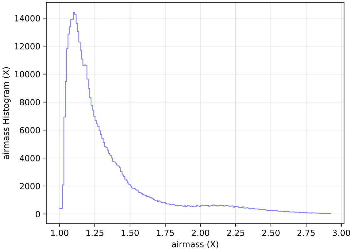
ddf_loaded_fl2_v3.4_10yrs All sky z band: airmass Histogram
