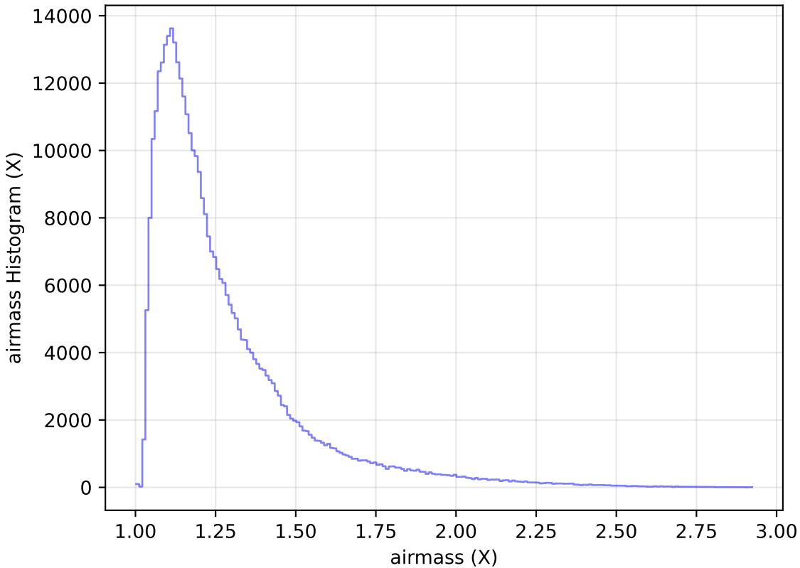
ddf_loaded_fl2_v3.4_10yrs All sky y band: airmass Histogram
