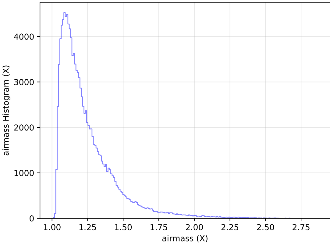
ddf_loaded_fl2_v3.4_10yrs All sky u band: airmass Histogram
