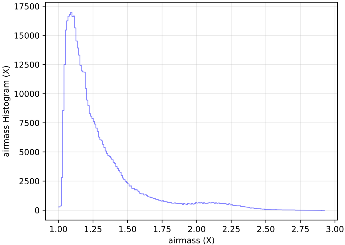
ddf_loaded_fl2_v3.4_10yrs All sky r band: airmass Histogram
