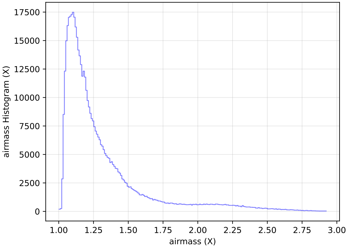
ddf_loaded_fl2_v3.4_10yrs All sky i band: airmass Histogram
