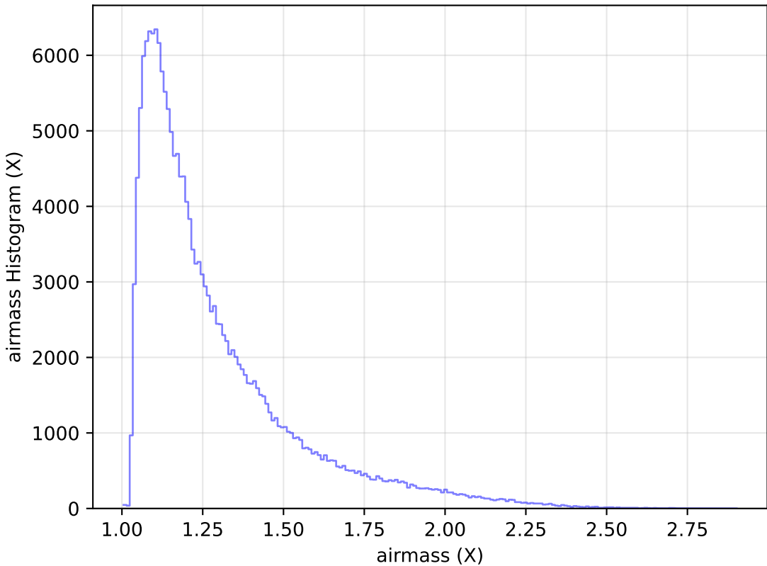
ddf_loaded_fl2_v3.4_10yrs All sky g band: airmass Histogram
