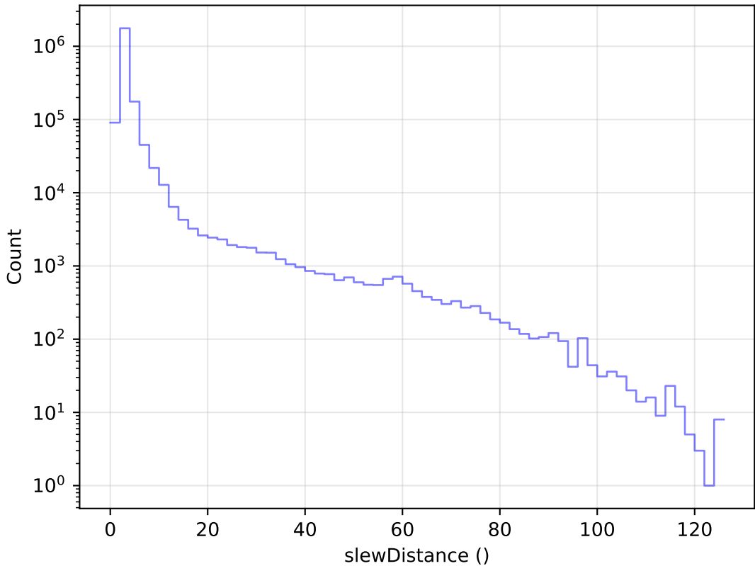
ddf_loaded_fl2_v3.4_10yrs All visits: Slew Distance Histogram
