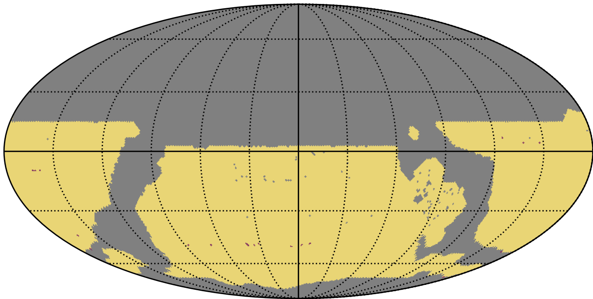
ddf_loaded_fl2_v3.4_10yrs WFD: RapidRevisits
