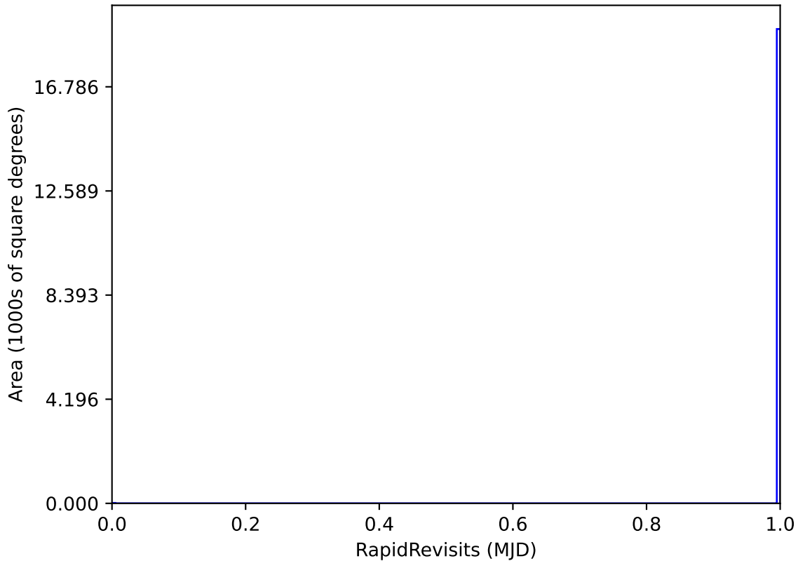
ddf_loaded_fl2_v3.4_10yrs WFD: RapidRevisits
