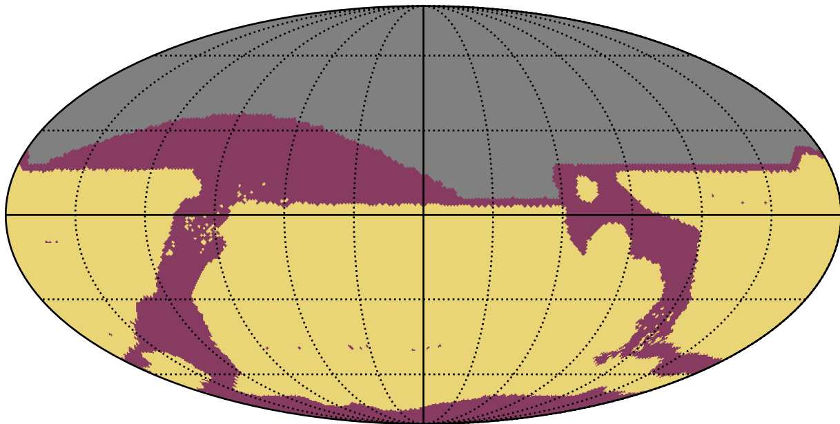
ddf_loaded_fl2_v3.4_10yrs All sky: RapidRevisits
