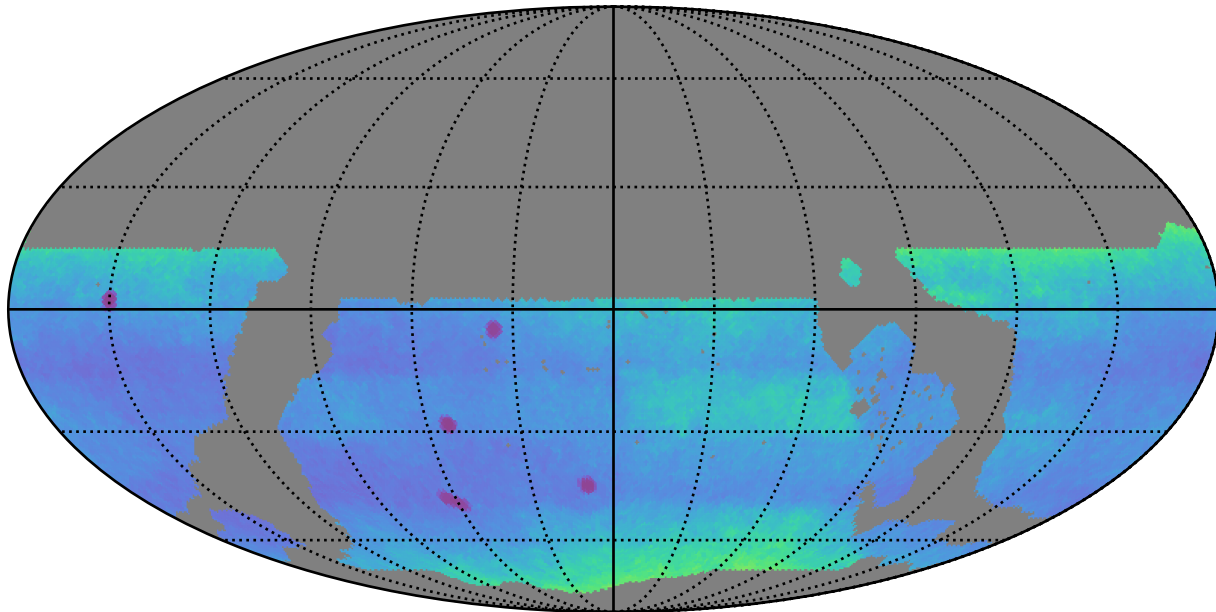
ddf_loaded_fl2_v3.4_10yrs WFD: Proper Motion Uncert @ 24.0
