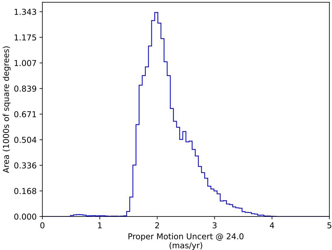
ddf_loaded_fl2_v3.4_10yrs WFD: Proper Motion Uncert @ 24.0
