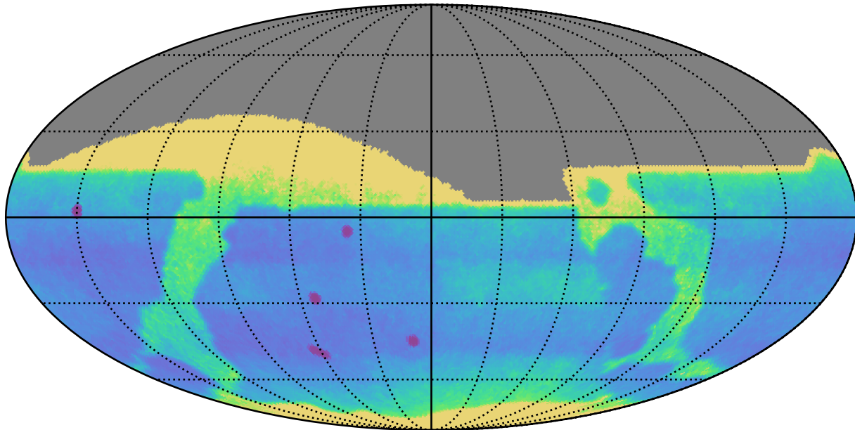
ddf_loaded_fl2_v3.4_10yrs All sky: Proper Motion Uncert @ 24.0
