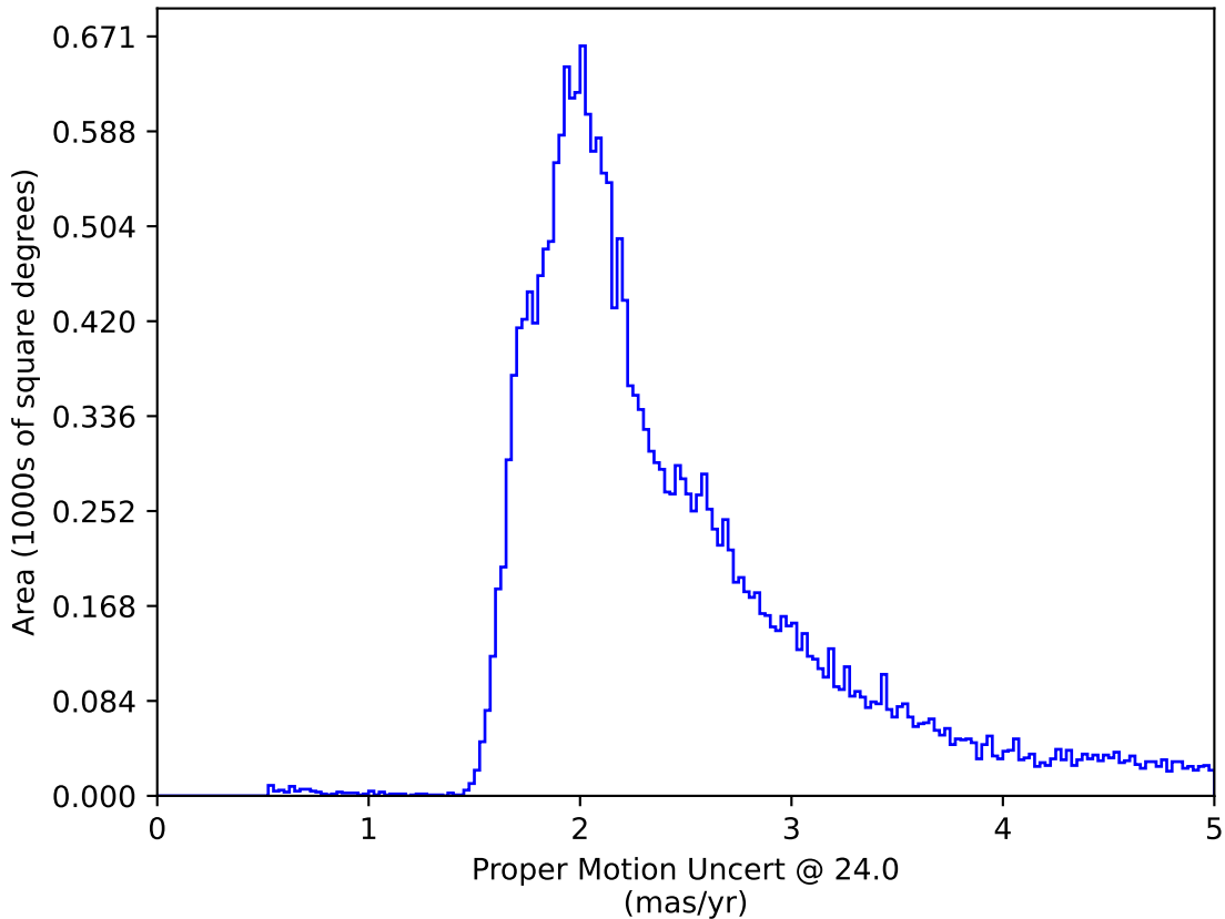
ddf_loaded_fl2_v3.4_10yrs All sky: Proper Motion Uncert @ 24.0
