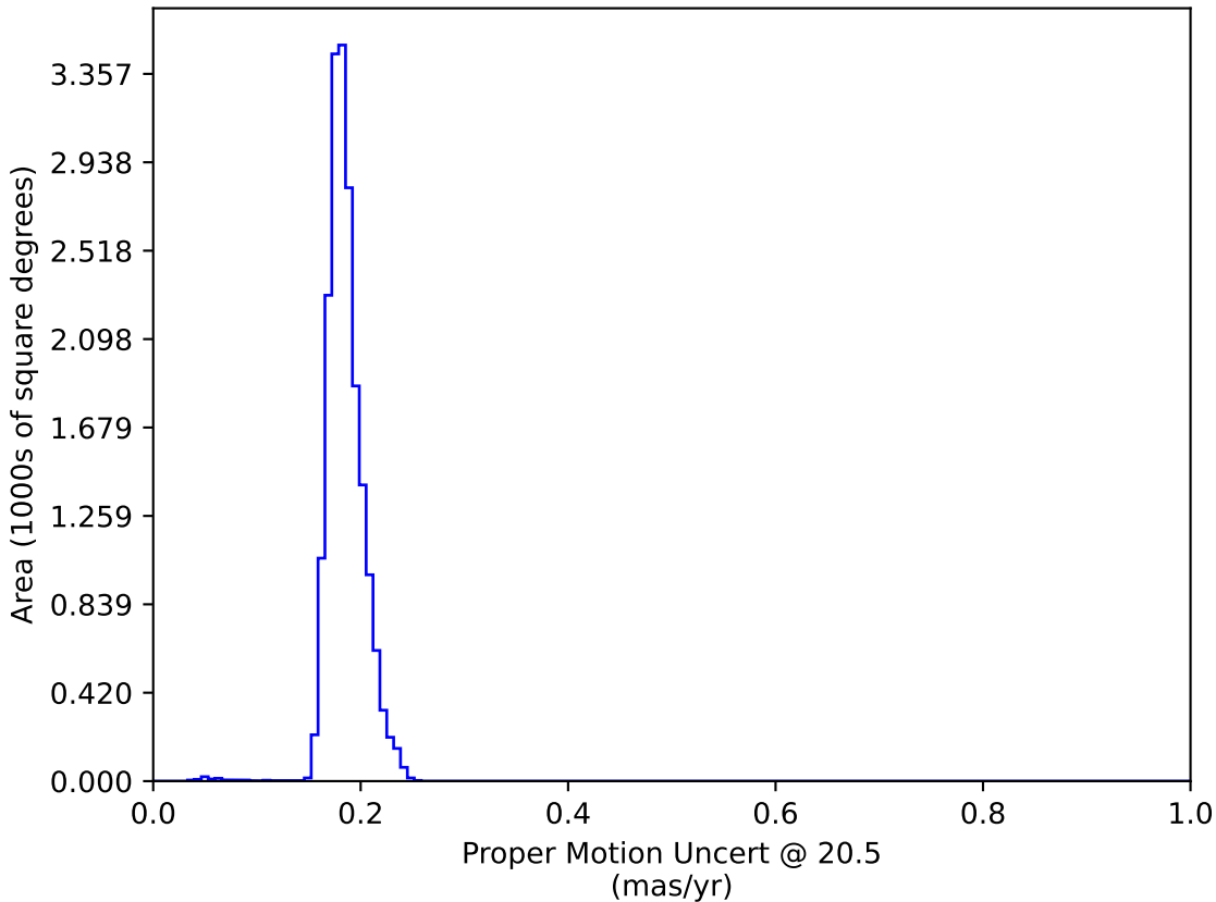
ddf_loaded_fl2_v3.4_10yrs WFD: Proper Motion Uncert @ 20.5
