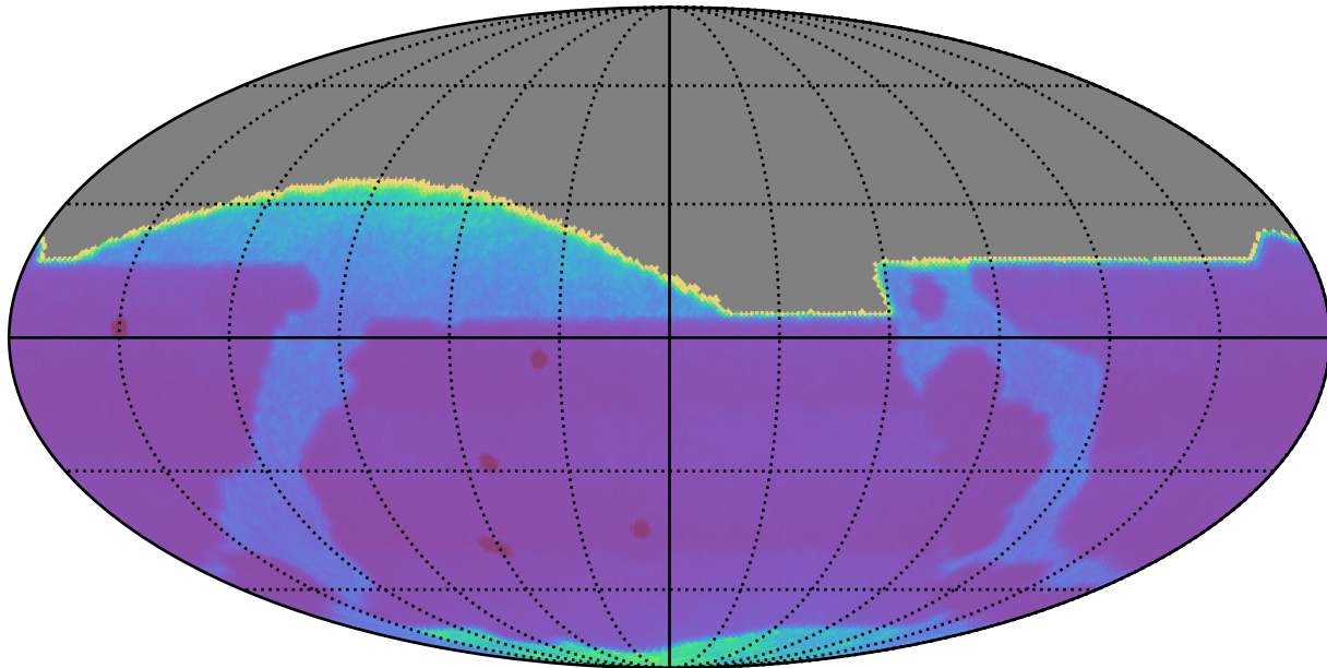
ddf_loaded_fl2_v3.4_10yrs All sky: Proper Motion Uncert @ 20.5
