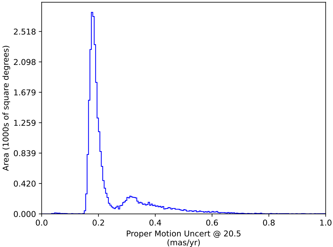
ddf_loaded_fl2_v3.4_10yrs All sky: Proper Motion Uncert @ 20.5
