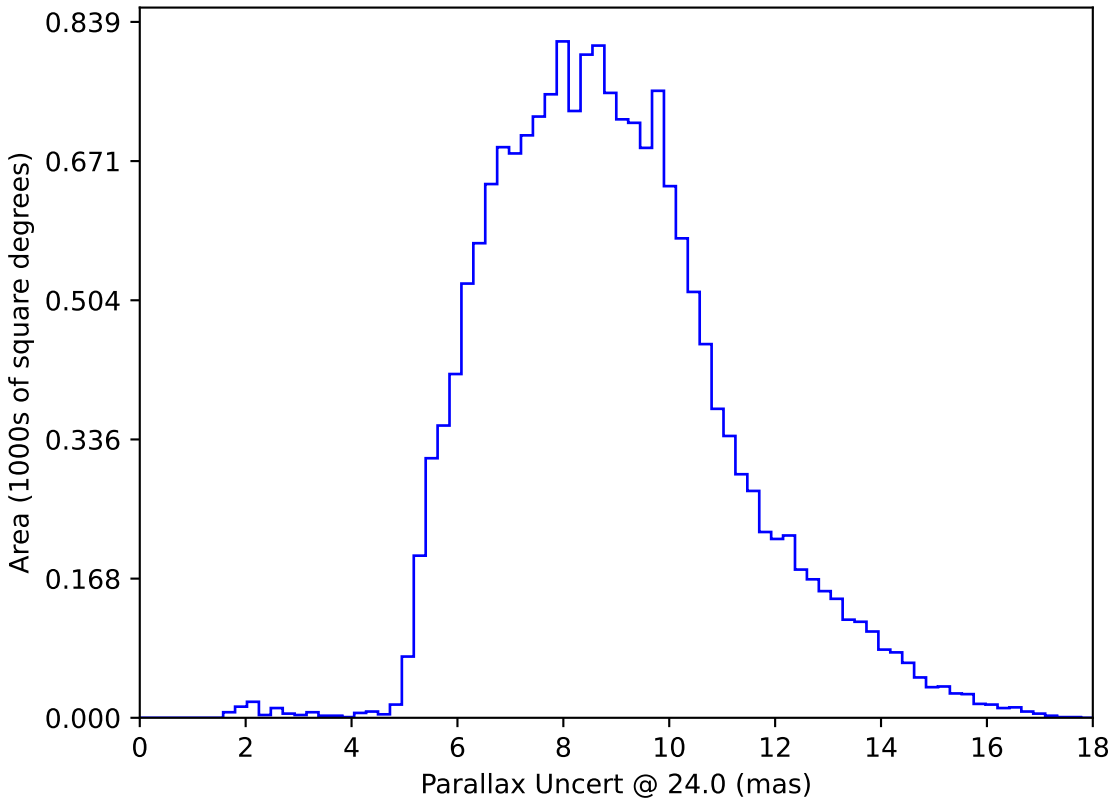
ddf_loaded_fl2_v3.4_10yrs WFD: Parallax Uncert @ 24.0
