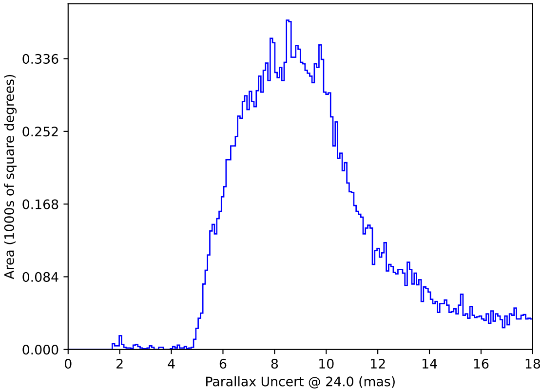
ddf_loaded_fl2_v3.4_10yrs All sky: Parallax Uncert @ 24.0
