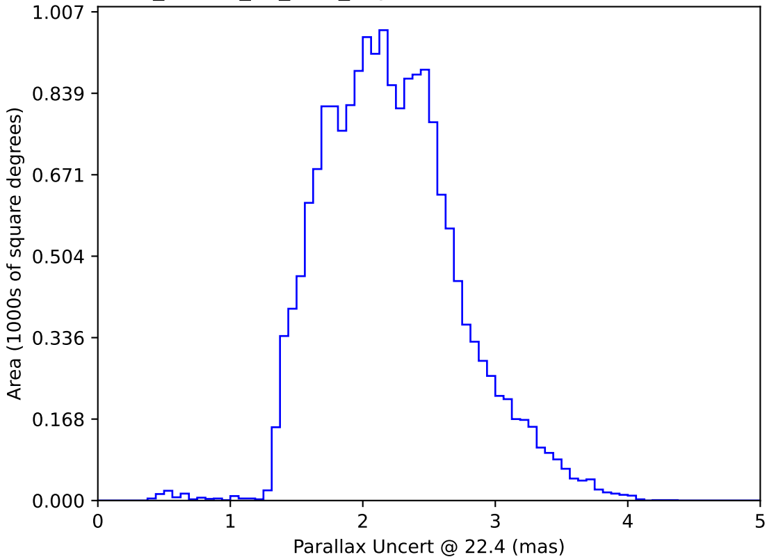
ddf_loaded_fl2_v3.4_10yrs WFD: Parallax Uncert @ 22.4
