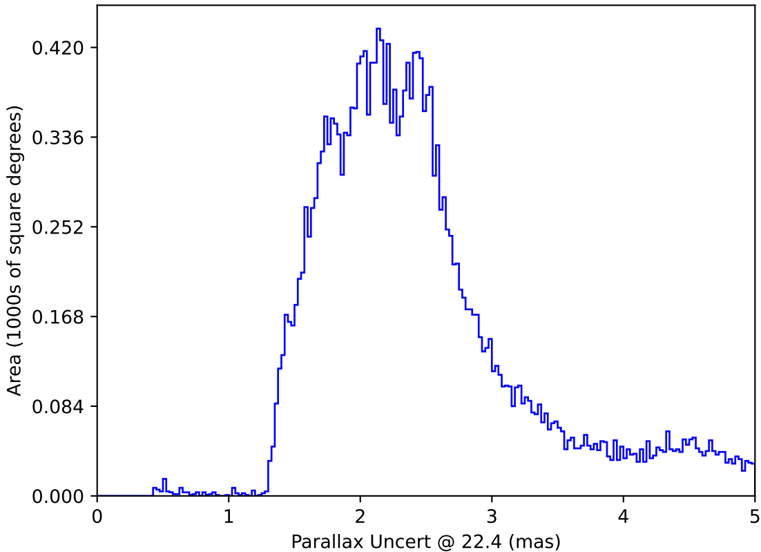
ddf_loaded_fl2_v3.4_10yrs All sky: Parallax Uncert @ 22.4
