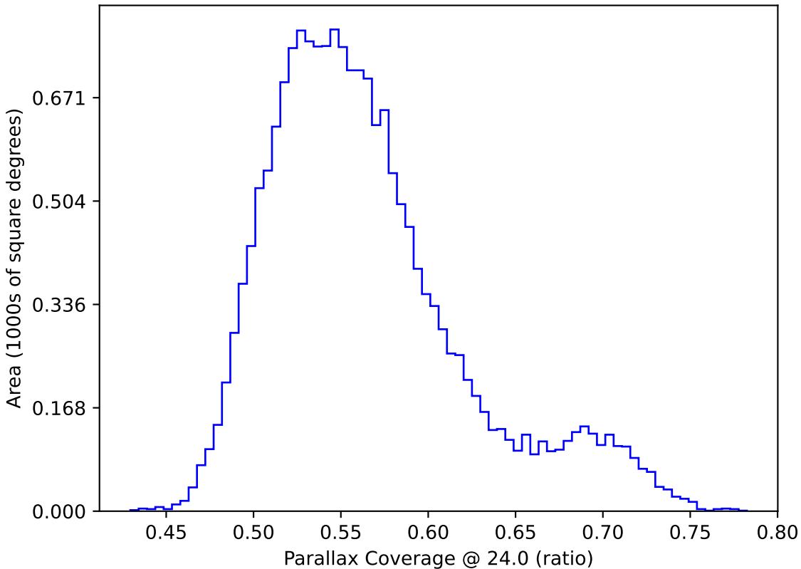
ddf_loaded_fl2_v3.4_10yrs WFD: Parallax Coverage @ 24.0
