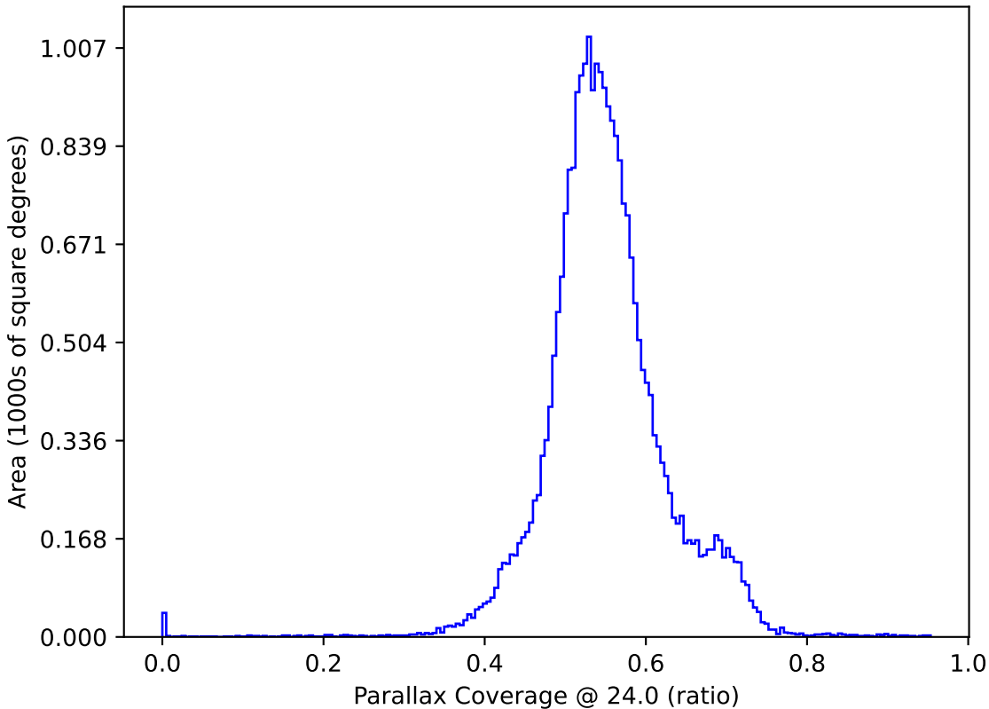
ddf_loaded_fl2_v3.4_10yrs All sky: Parallax Coverage @ 24.0
