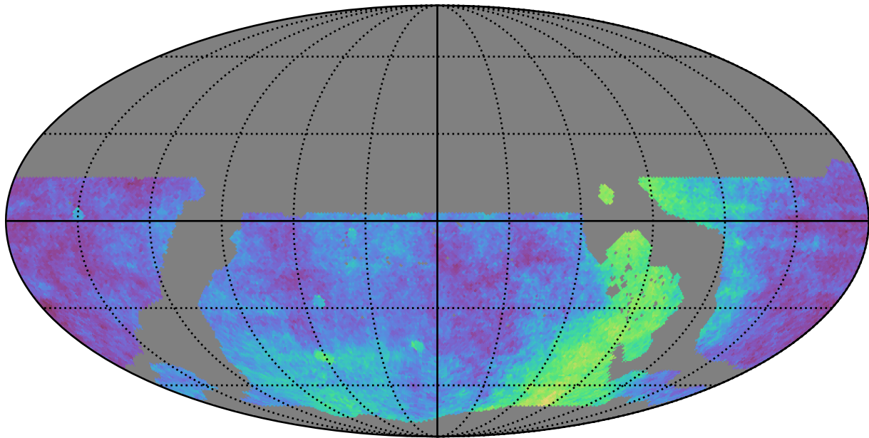
ddf_loaded_fl2_v3.4_10yrs WFD: Parallax Coverage @ 22.4
