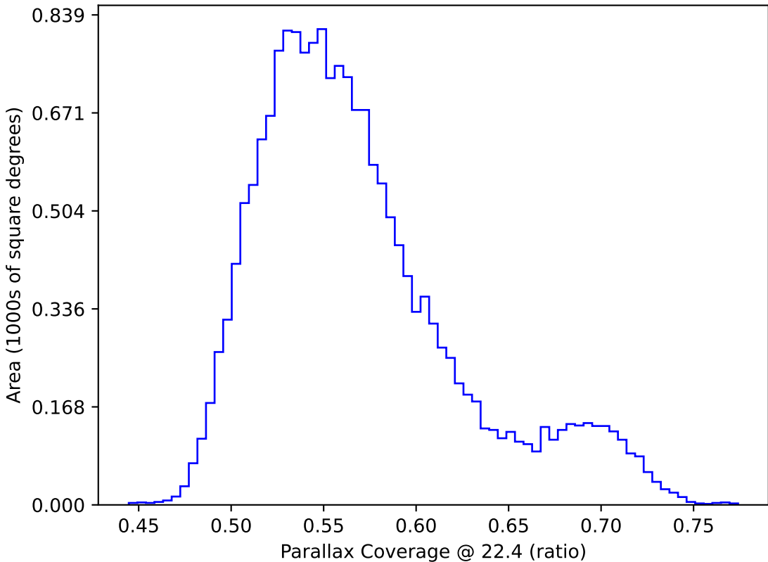
ddf_loaded_fl2_v3.4_10yrs WFD: Parallax Coverage @ 22.4
