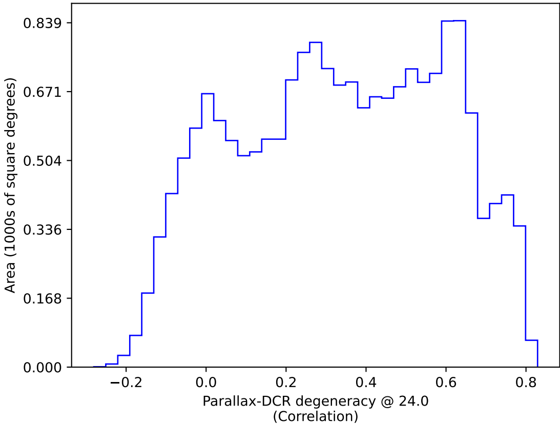
ddf_loaded_fl2_v3.4_10yrs WFD: Parallax-DCR degeneracy @ 24.0
