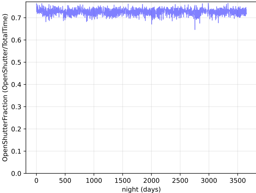
ddf_loaded_fl2_v3.4_10yrs Per night: OpenShutterFraction
