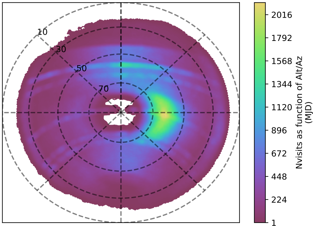
ddf_loaded_fl2_v3.4_10yrs z band: Nvisits as function of Alt/Az
