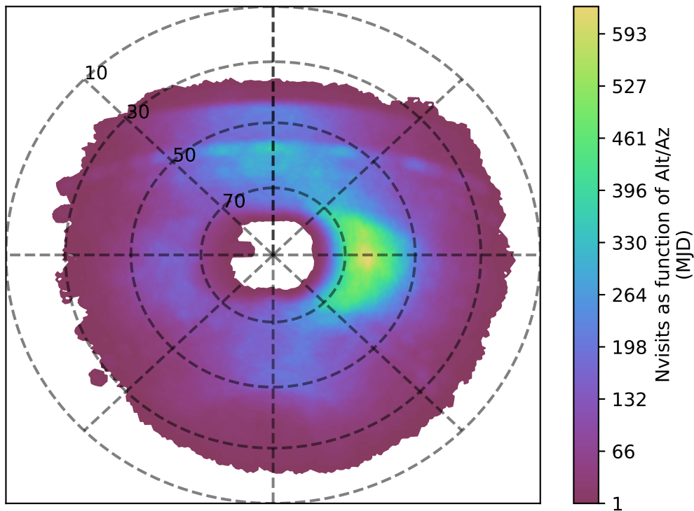
ddf_loaded_fl2_v3.4_10yrs u band: Nvisits as function of Alt/Az
