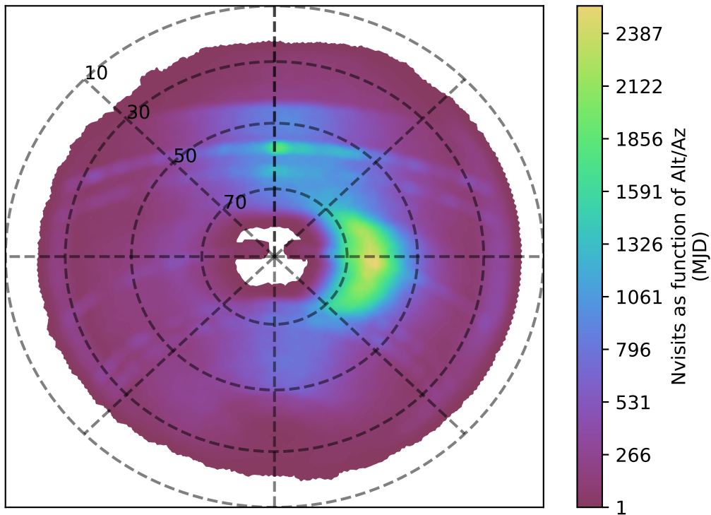
ddf_loaded_fl2_v3.4_10yrs i band: Nvisits as function of Alt/Az
