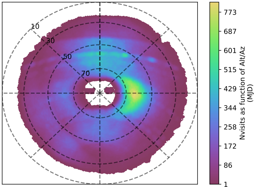
ddf_loaded_fl2_v3.4_10yrs g band: Nvisits as function of Alt/Az
