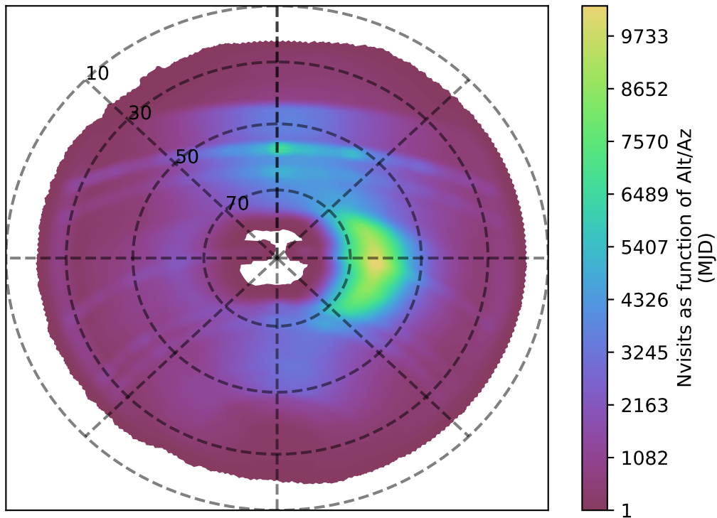
ddf_loaded_fl2_v3.4_10yrs all bands: Nvisits as function of Alt/Az
