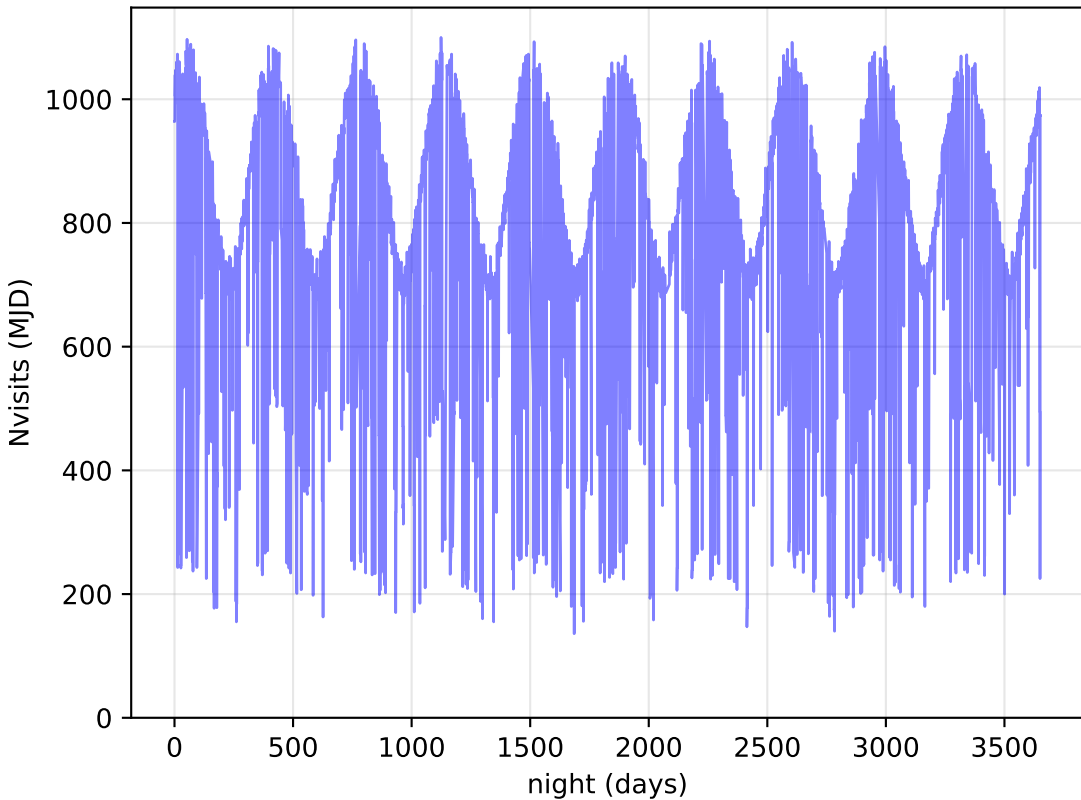
ddf_loaded_fl2_v3.4_10yrs All visits: Nvisits
