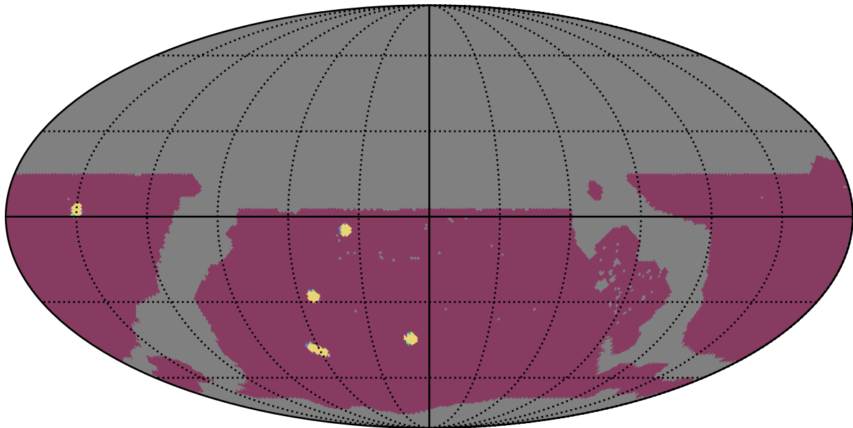
ddf_loaded_fl2_v3.4_10yrs WFD: NumberOfQuickRevisits
