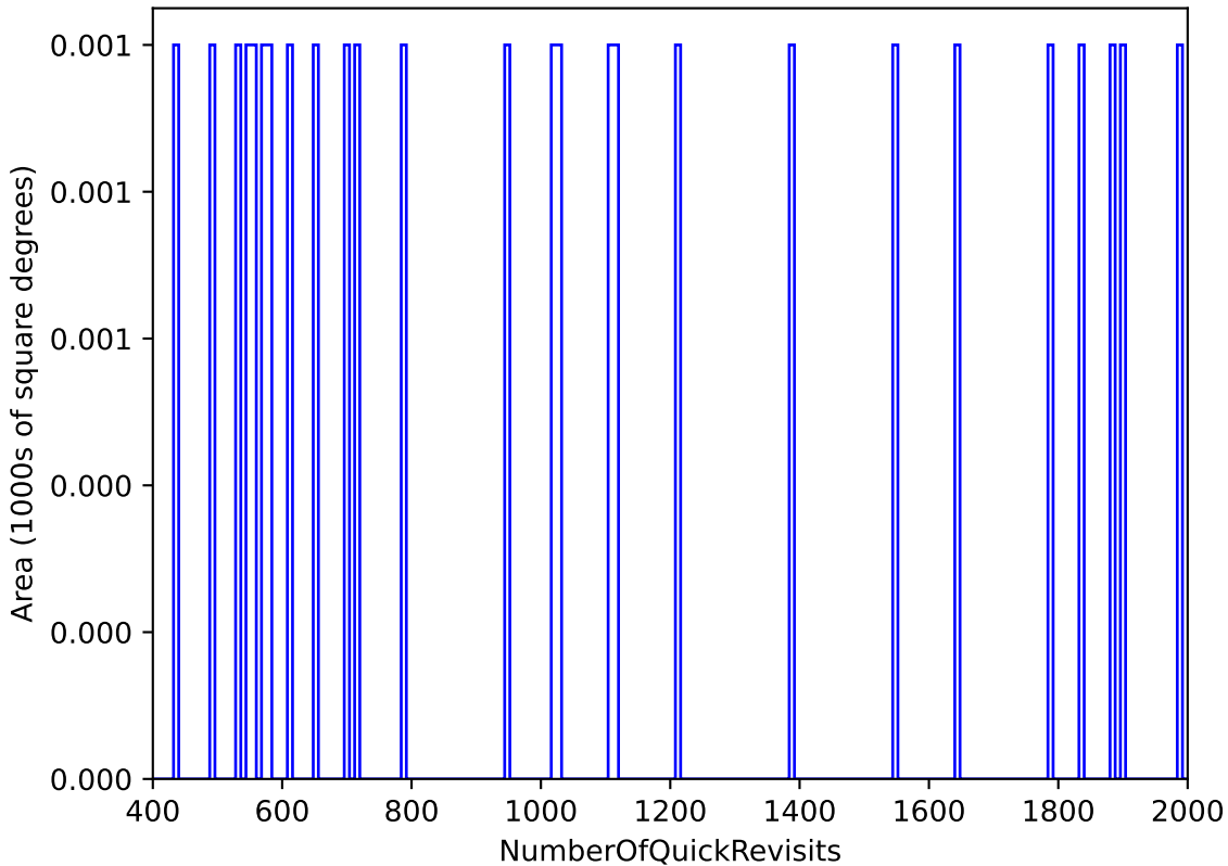
ddf_loaded_fl2_v3.4_10yrs All sky: NumberOfQuickRevisits
