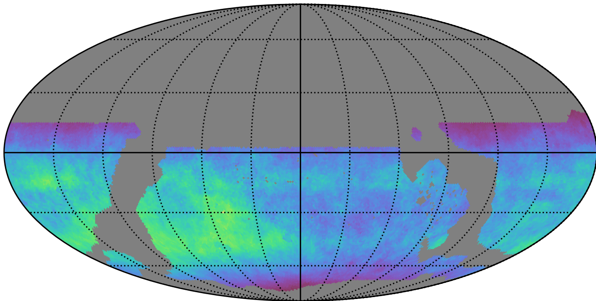
ddf_loaded_fl2_v3.4_10yrs WFD z band: Normalized Teff
