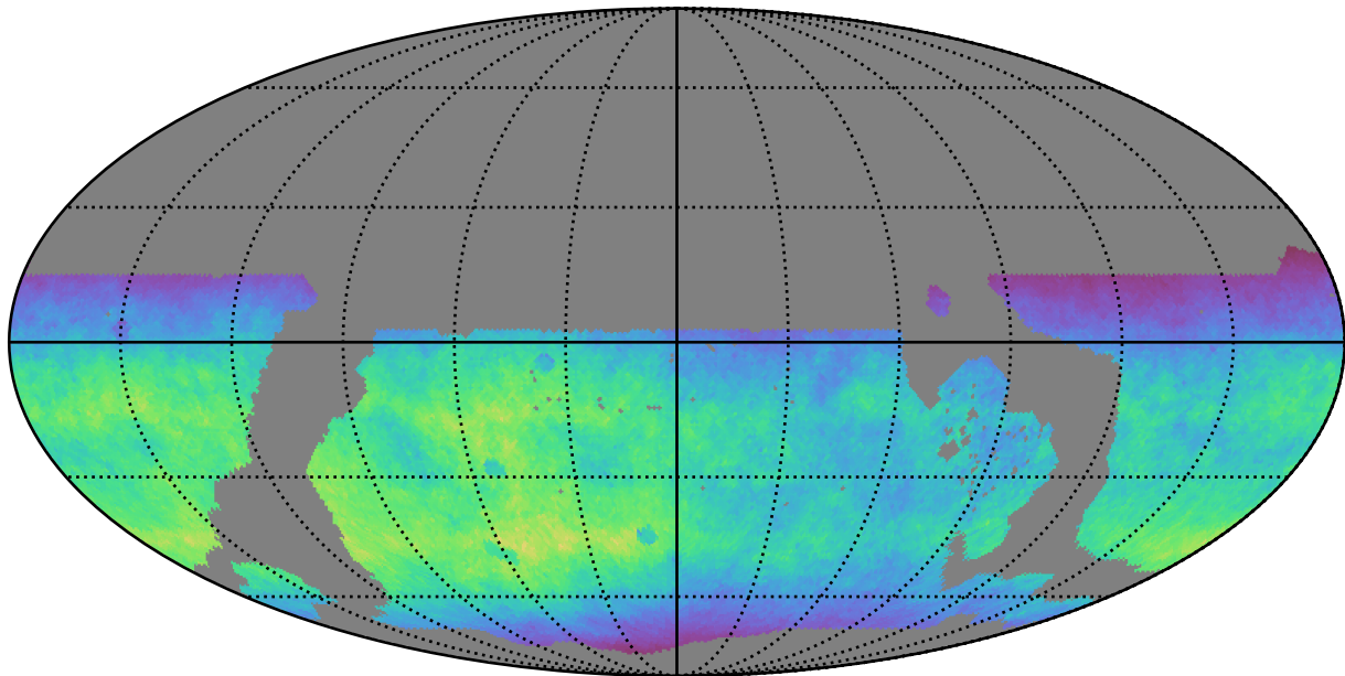
ddf_loaded_fl2_v3.4_10yrs WFD y band: Normalized Teff
