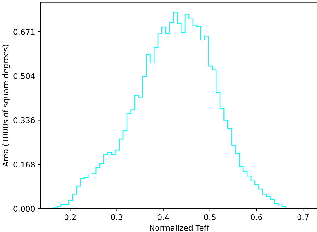
ddf_loaded_fl2_v3.4_10yrs WFD u band: Normalized Teff
