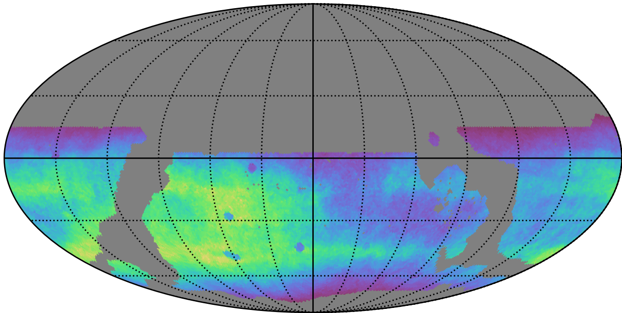
ddf_loaded_fl2_v3.4_10yrs WFD r band: Normalized Teff
