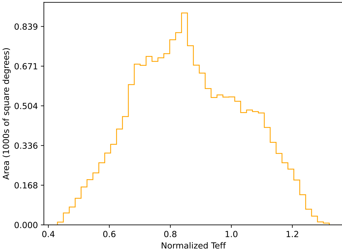
ddf_loaded_fl2_v3.4_10yrs WFD r band: Normalized Teff
