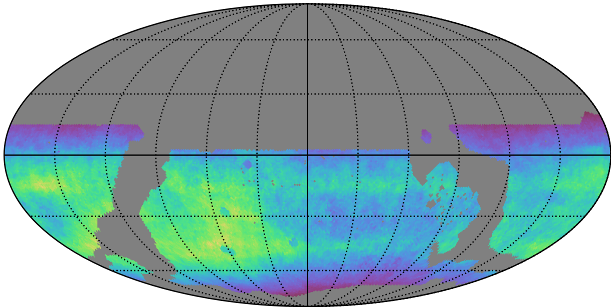
ddf_loaded_fl2_v3.4_10yrs WFD i band: Normalized Teff
