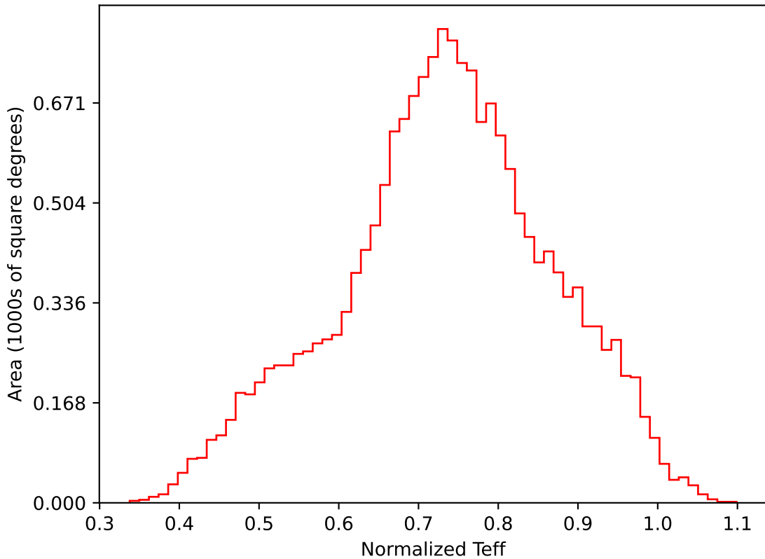
ddf_loaded_fl2_v3.4_10yrs WFD i band: Normalized Teff
